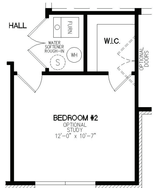
OPTION UTILITY LOCATION ON SLAB
